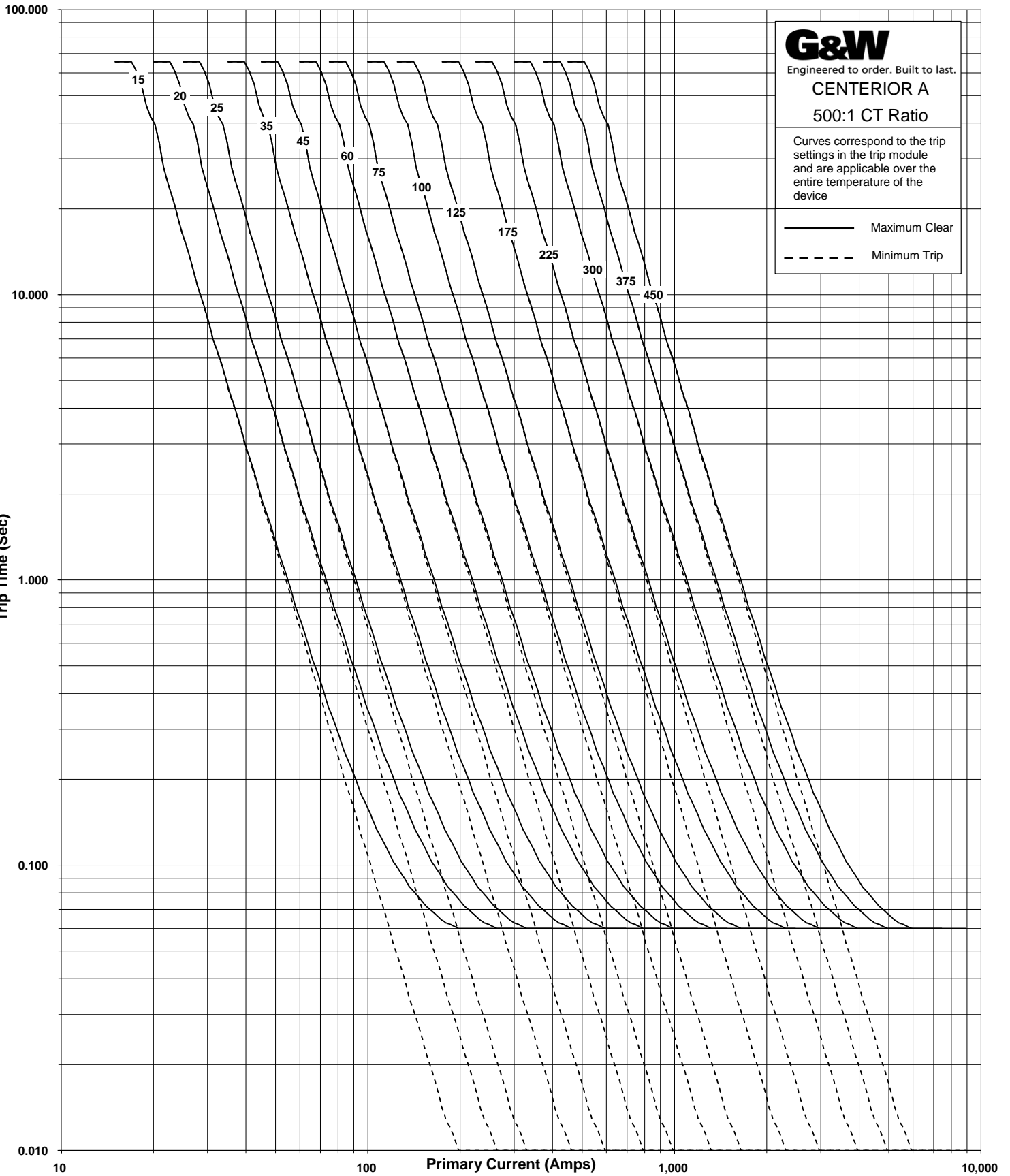
TIME - CURRENT CHARACTERISTIC CURVES FOR VI CONTROLS
